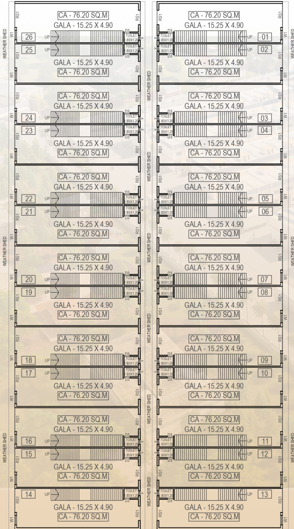
GROUND FLOOR PLAN (BUILDING- 1,2)
